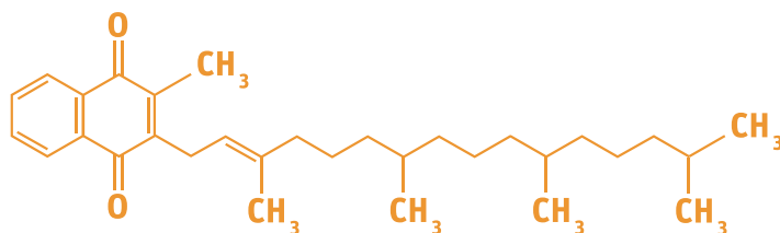
K 1 Phylloquinone
