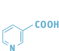
Nicotinic Acid
